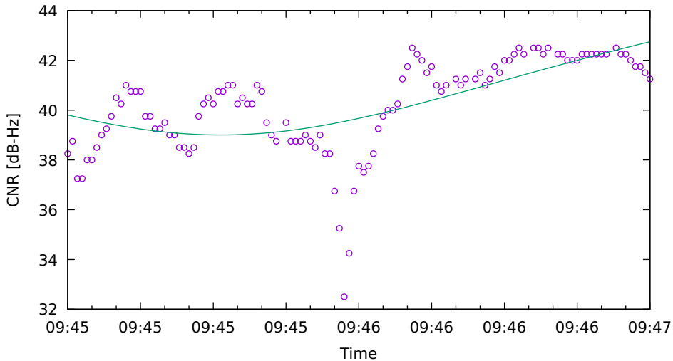
CNR fit for G32 on SamsungS20 - drive 4 (DOY263)
