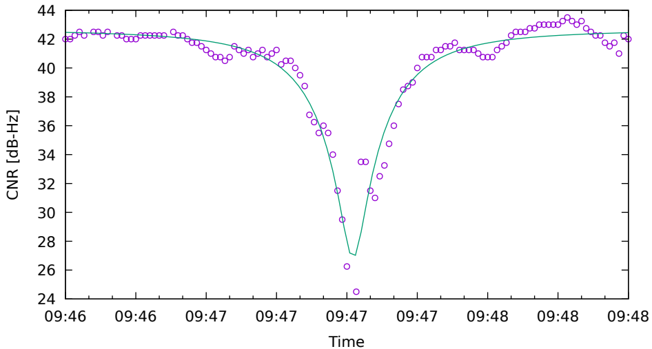
CNR fit for G32 on SamsungS20 - drive 5 (DOY263)
