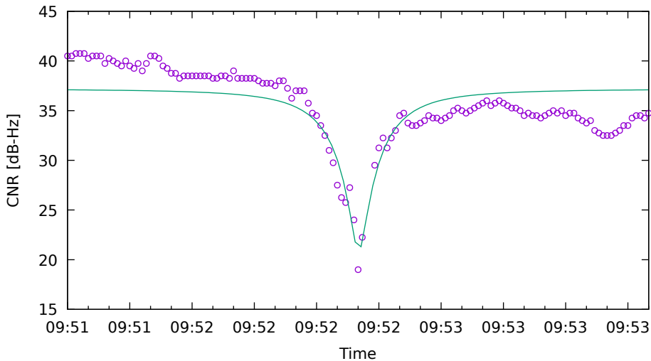
CNR fit for G32 on SamsungS20 - drive 8 (DOY263)
