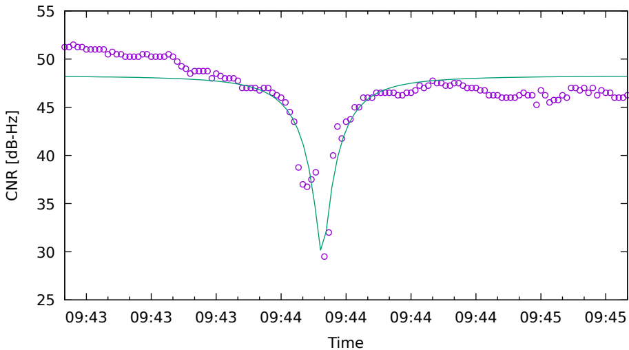
CNR fit for R02 on SamsungS20 - drive 3 (DOY263)
