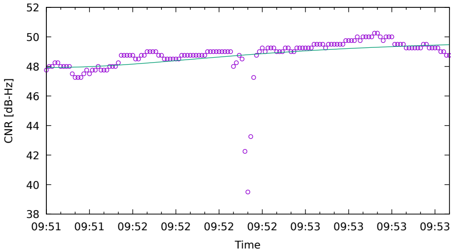
CNR fit for R17 on SamsungS20 - drive 8 (DOY263)
