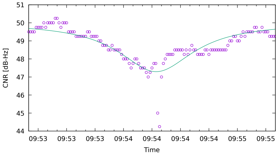
CNR fit for R17 on SamsungS20 - drive 9 (DOY263)
