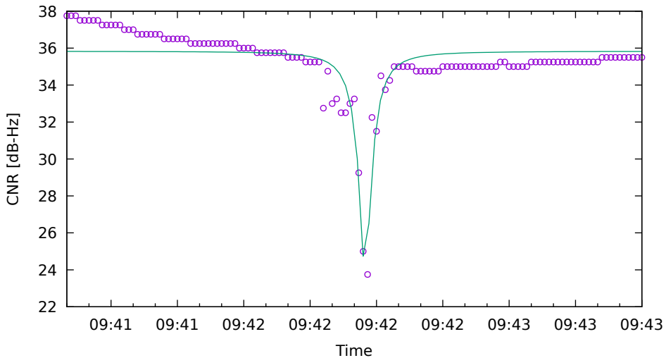
CNR fit for E04 on Xiaomi11T - drive 2 (DOY263)
