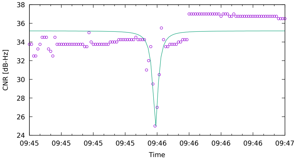
CNR fit for E11 on Xiaomi11T - drive 4 (DOY263)
