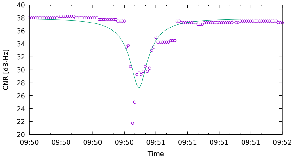
CNR fit for E11 on Xiaomi11T - drive 7 (DOY263)
