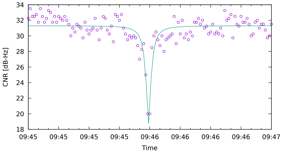
CNR fit for E12 on Xiaomi11T - drive 4 (DOY263)
