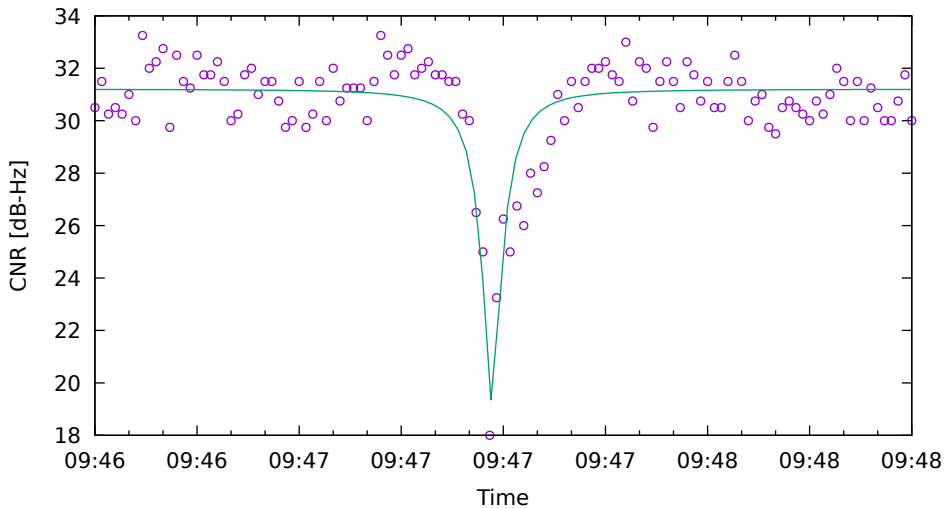
CNR fit for E12 on Xiaomi11T - drive 5 (DOY263)
