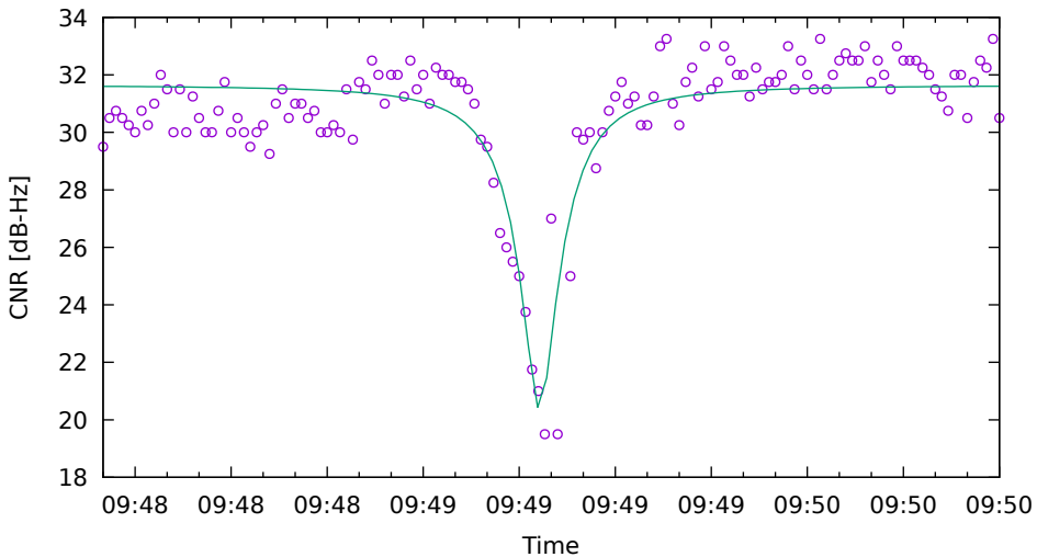
CNR fit for E12 on Xiaomi11T - drive 6 (DOY263)
