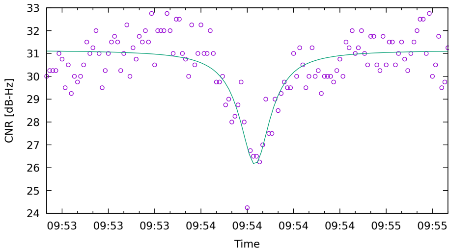
CNR fit for E12 on Xiaomi11T - drive 9 (DOY263)
