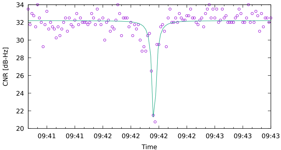
CNR fit for E19 on Xiaomi11T - drive 2 (DOY263)
