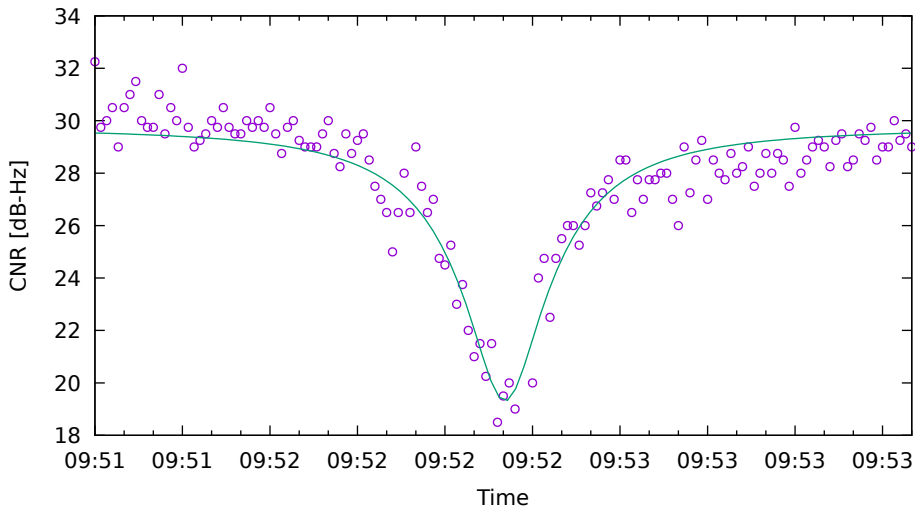
CNR fit for E19 on Xiaomi11T - drive 8 (DOY263)
