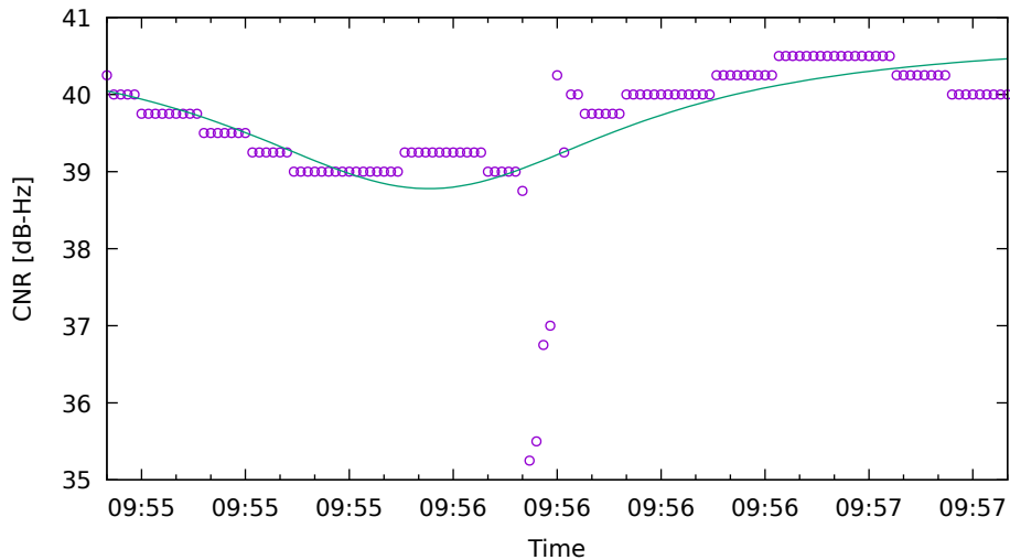
CNR fit for G01 on Xiaomi11T - drive 10 (DOY263)
