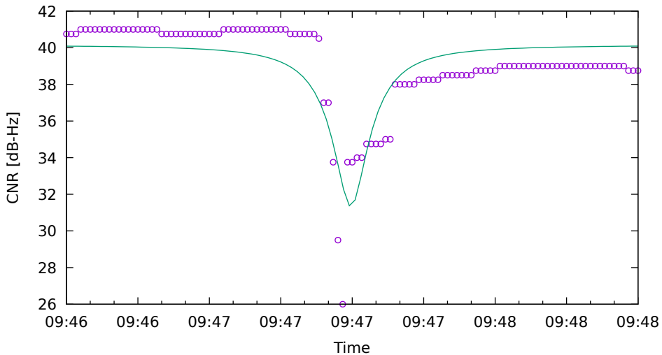
CNR fit for G01 on Xiaomi11T - drive 5 (DOY263)
