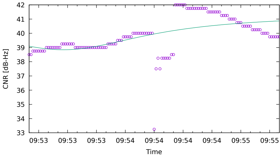
CNR fit for G01 on Xiaomi11T - drive 9 (DOY263)
