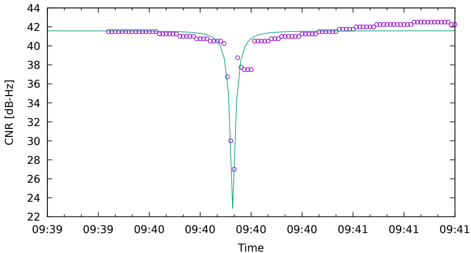
CNR fit for G03 on Xiaomi11T - drive 1 (DOY263)
