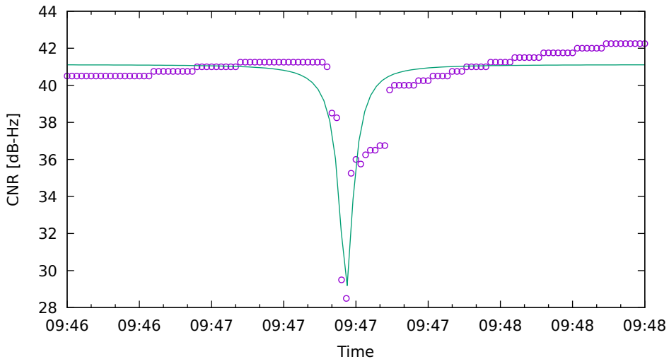
CNR fit for G03 on Xiaomi11T - drive 5 (DOY263)
