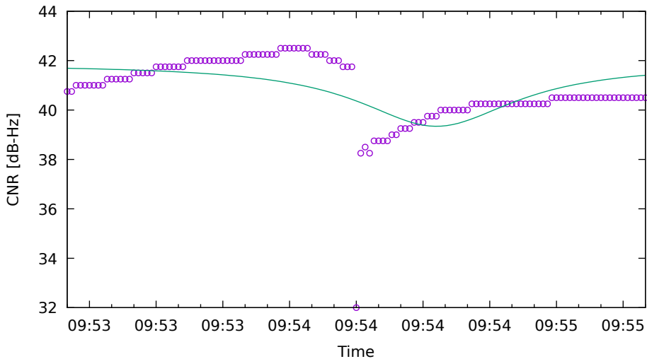
CNR fit for G03 on Xiaomi11T - drive 9 (DOY263)
