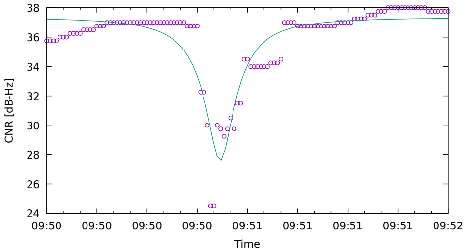
CNR fit for G08 on Xiaomi11T - drive 7 (DOY263)
