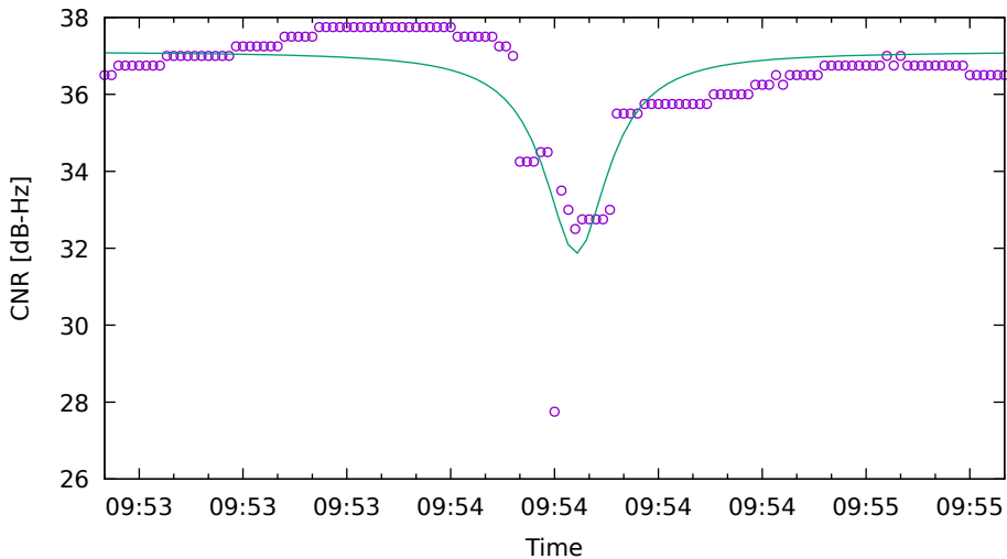
CNR fit for G08 on Xiaomi11T - drive 9 (DOY263)
