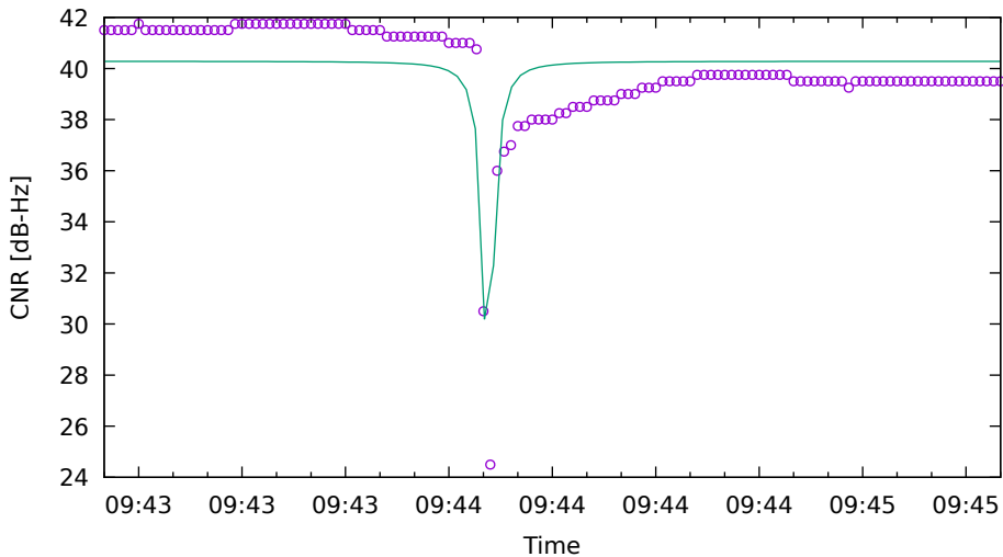
CNR fit for G17 on Xiaomi11T - drive 3 (DOY263)
