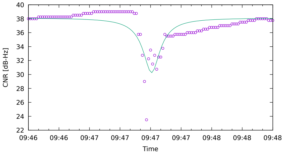
CNR fit for G17 on Xiaomi11T - drive 5 (DOY263)
