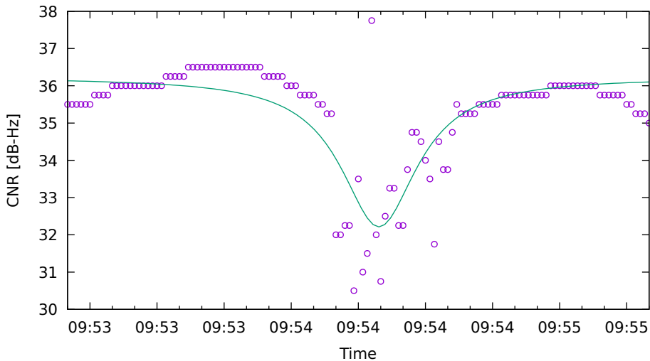
CNR fit for G17 on Xiaomi11T - drive 9 (DOY263)
