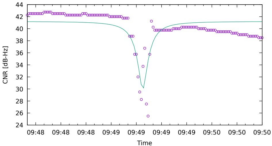
CNR fit for G21 on Xiaomi11T - drive 6 (DOY263)
