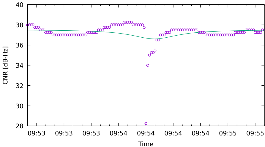
CNR fit for G21 on Xiaomi11T - drive 9 (DOY263)
