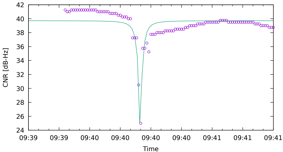
CNR fit for G32 on Xiaomi11T - drive 1 (DOY263)
