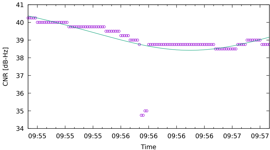
CNR fit for G32 on Xiaomi11T - drive 10 (DOY263)
