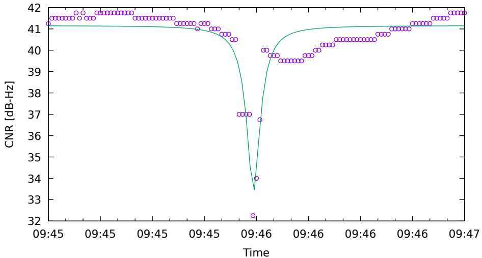
CNR fit for G32 on Xiaomi11T - drive 4 (DOY263)
