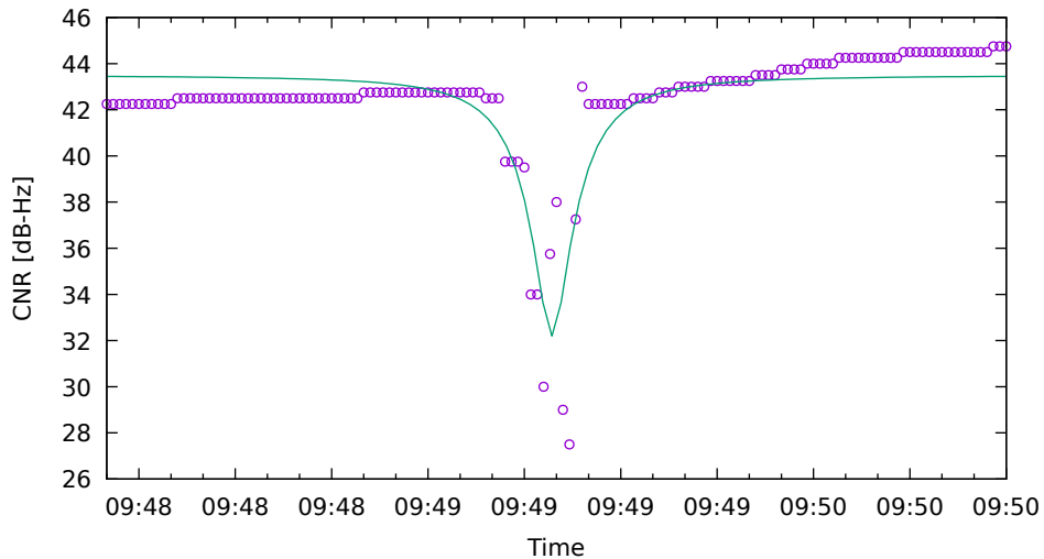
CNR fit for G32 on Xiaomi11T - drive 6 (DOY263)
