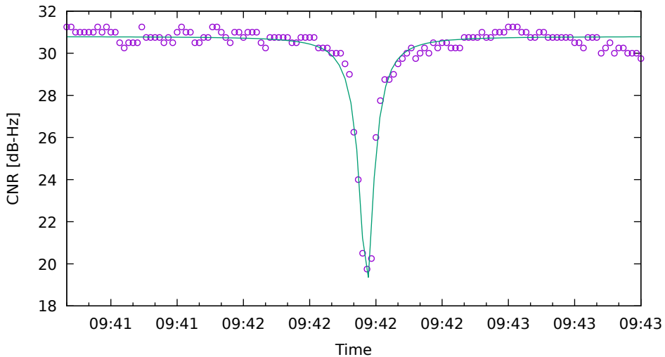
CNR fit for C09 on XiaomiMi8 - drive 2 (DOY263)
