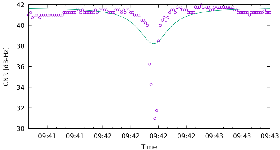
CNR fit for C11 on XiaomiMi8 - drive 2 (DOY263)
