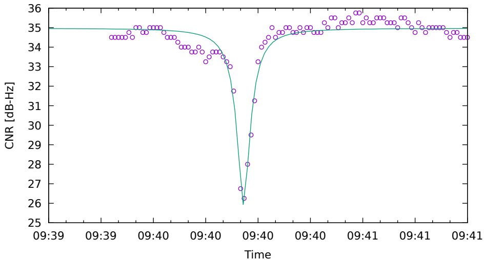
CNR fit for C12 on XiaomiMi8 - drive 1 (DOY263)
