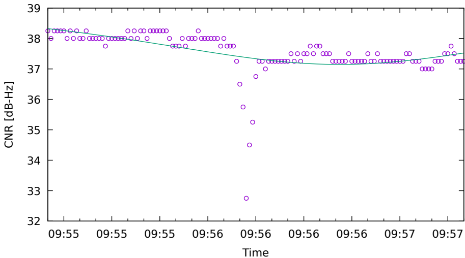
CNR fit for C12 on XiaomiMi8 - drive 10 (DOY263)
