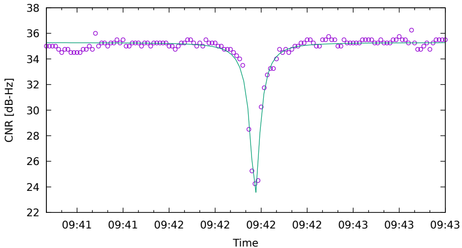
CNR fit for C12 on XiaomiMi8 - drive 2 (DOY263)
