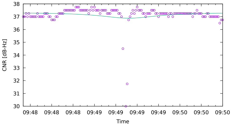
CNR fit for C12 on XiaomiMi8 - drive 6 (DOY263)
