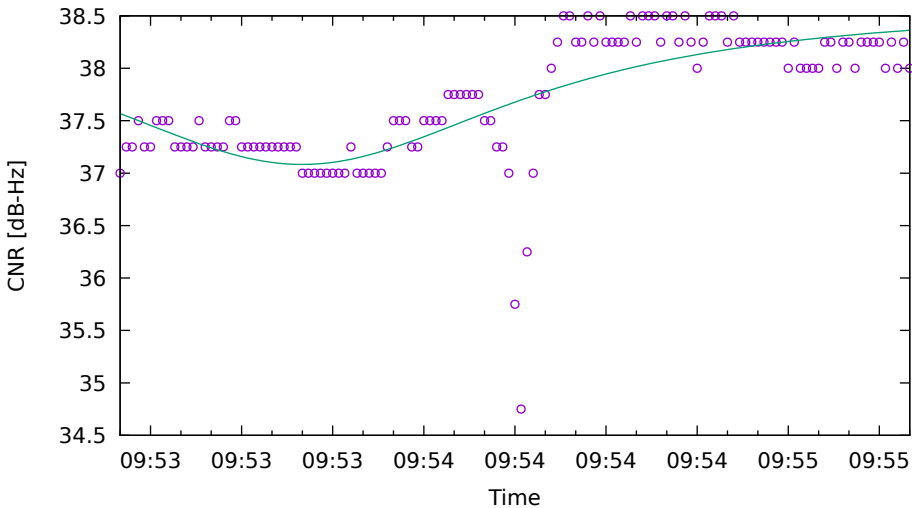
CNR fit for C12 on XiaomiMi8 - drive 9 (DOY263)
