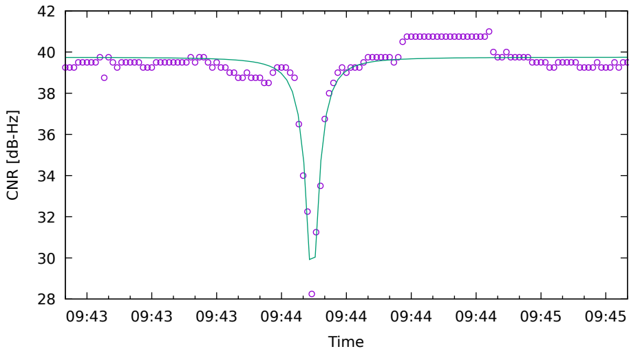
CNR fit for C28 on XiaomiMi8 - drive 3 (DOY263)
