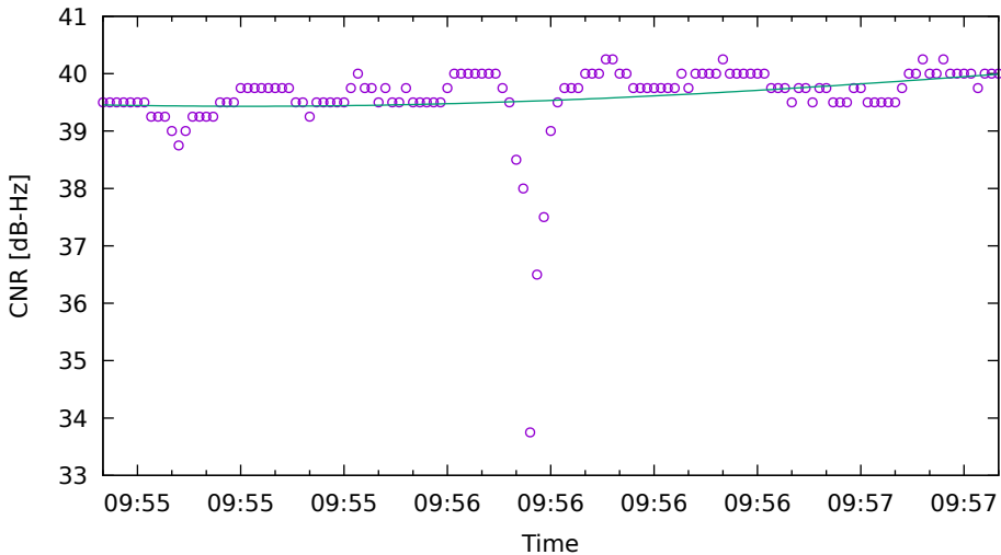
CNR fit for C34 on XiaomiMi8 - drive 10 (DOY263)
