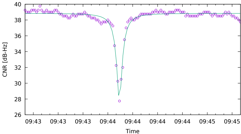
CNR fit for C34 on XiaomiMi8 - drive 3 (DOY263)
