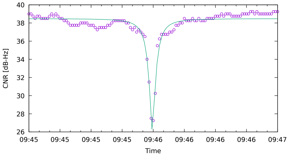
CNR fit for C34 on XiaomiMi8 - drive 4 (DOY263)
