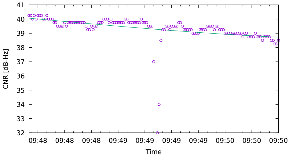
CNR fit for C34 on XiaomiMi8 - drive 6 (DOY263)
