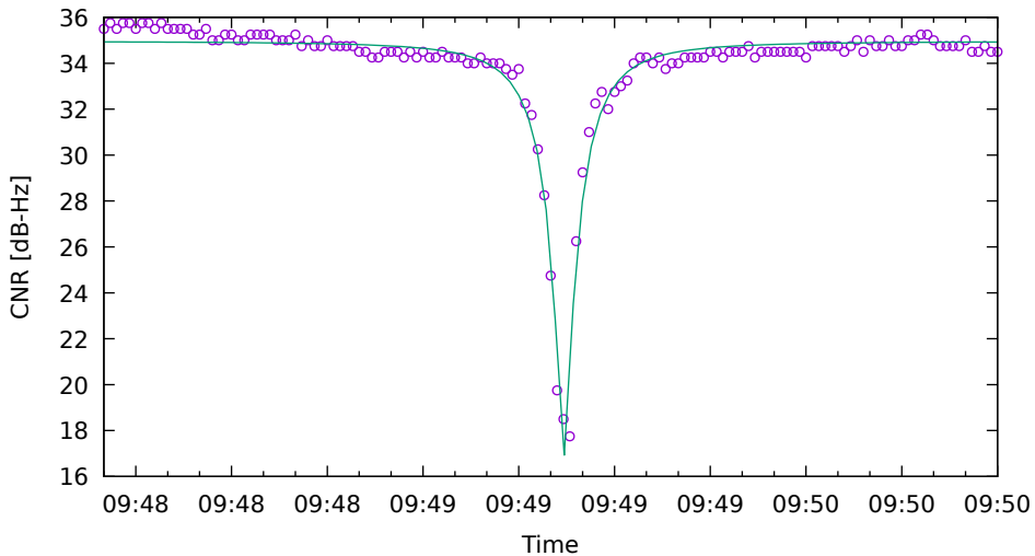
CNR fit for E04 on XiaomiMi8 - drive 6 (DOY263)
