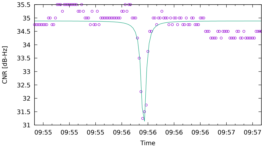
CNR fit for E19 on XiaomiMi8 - drive 10 (DOY263)
