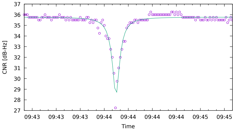
CNR fit for E19 on XiaomiMi8 - drive 3 (DOY263)
