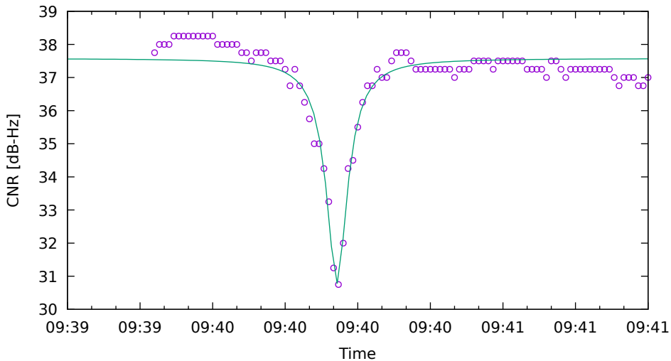
CNR fit for E33 on XiaomiMi8 - drive 1 (DOY263)
