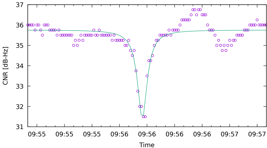
CNR fit for E33 on XiaomiMi8 - drive 10 (DOY263)
