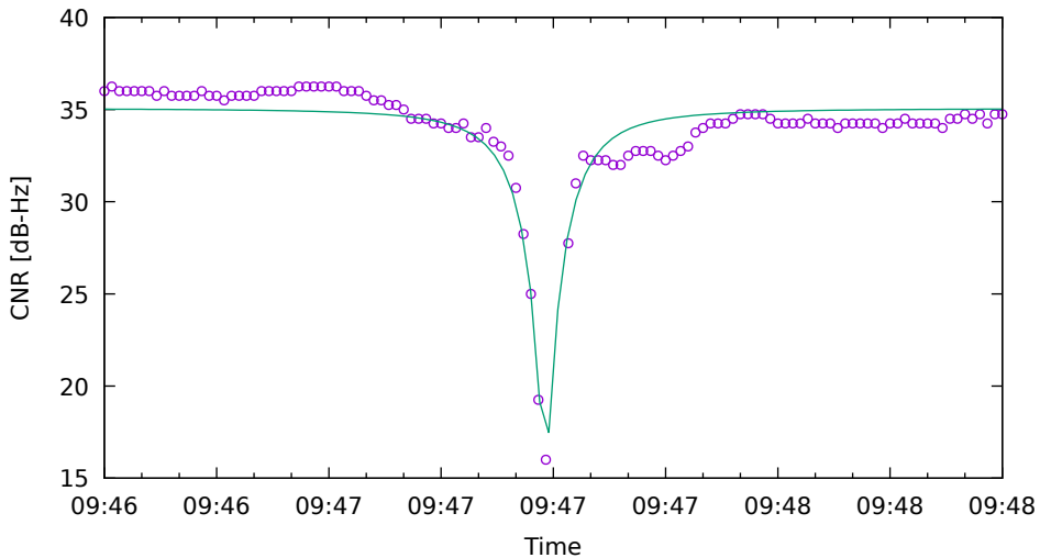
CNR fit for E33 on XiaomiMi8 - drive 5 (DOY263)
